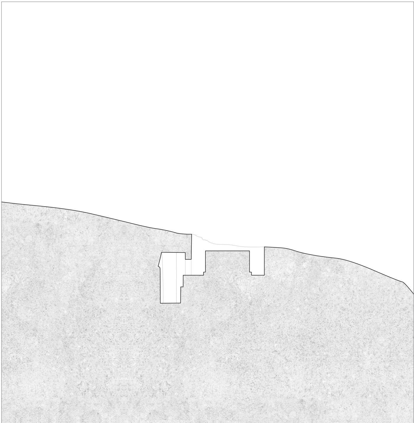
Dagmawi Lalibela (Ambager Complex) Section OO (2017)
